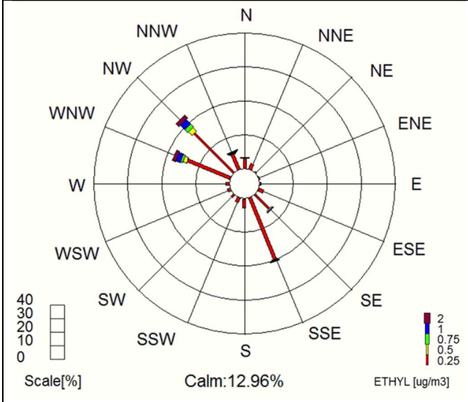
Pollution Rose for EthylBenzene ( \mu\text{g}/\text{m}^3 ) 01/06/2021 00:00 – 31/05/2022 24:00 Station O.L. Volos AVG: 15min
