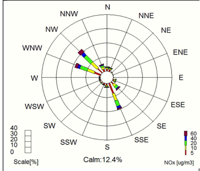
Pollution Rose for NO x ( \mu\text{g}/\text{m}^3 ) 01/06/2021 00:00 – 31/05/2022 24:00 Station O.L. Volos AVG: 5min
