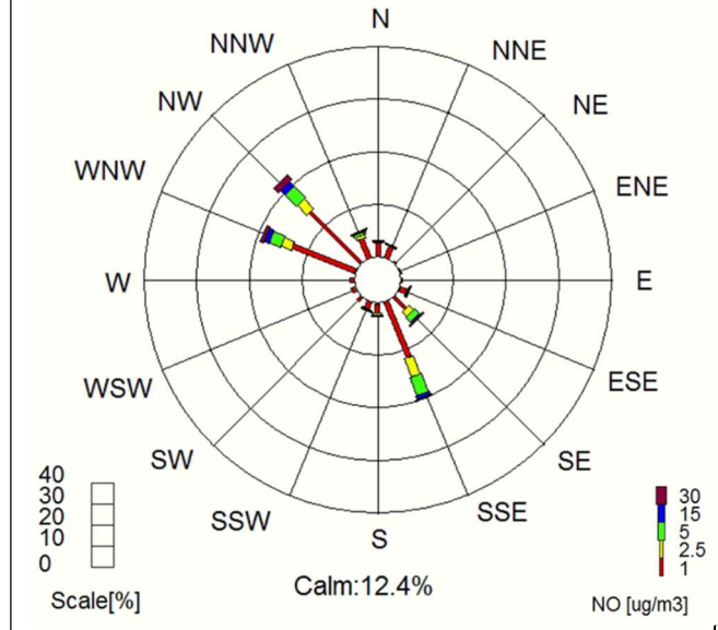
Pollution Rose for NO ( \mu\text{g}/\text{m}^3 ) 01/06/2021 00:00 – 31/05/2022 24:00 Station O.L. Volos AVG: 5min
