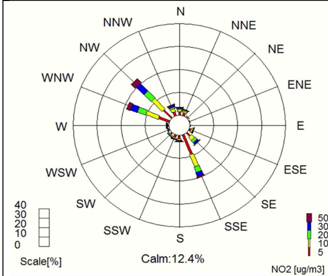
Pollution Rose for NO 2 ( \mu\text{g}/\text{m}^3 ) 01/06/2021 00:00 – 31/05/2022 24:00 Station O.L. Volos AVG: 5min
