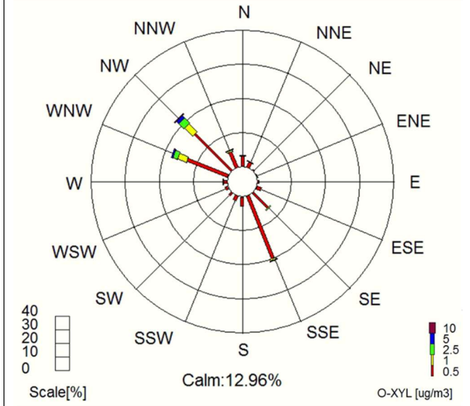
Pollution Rose for o-Xylene ( \mu\text{g}/\text{m}^3 ) 01/06/2021 00:00 – 31/05/2022 24:00 Station O.L. Volos AVG: 15min
