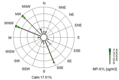
Periodic Pollution Rose VOLOS For MP-XYL[ug/m3] 31/05/2018 24:00-31/05/2019 24:00 Station:VOLOS AVG:5 Min
