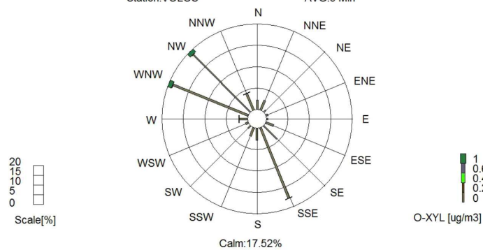
Periodic Pollution Rose VOLOS For O-XYL[ug/m3] 31/05/2018 24:00-31/05/2019 24:00 Station:VOLOS AVG:5 Min
