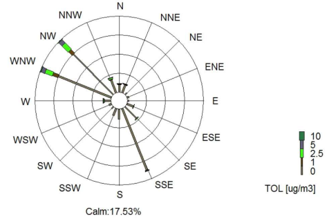
Periodic Pollution Rose VOLOS For TOL[ug/m3] 31/05/2018 24:00-31/05/2019 24:00 Station:VOLOS AVG:5 Min
