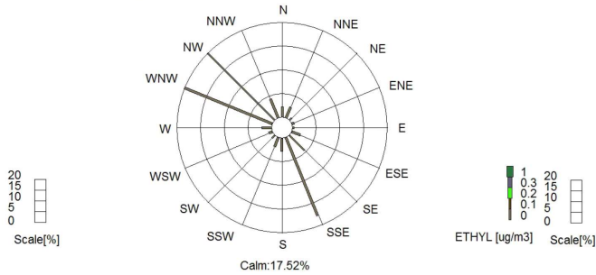
Periodic Pollution Rose VOLOS For ETHYL[ug/m3] 31/05/2018 24:00-31/05/2019 24:00 Station:VOLOS AVG:5 Min
