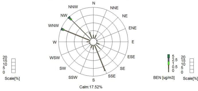
Periodic Pollution Rose VOLOS For BEN[ug/m3] 31/05/2018 24:00-31/05/2019 24:00 Station:VOLOS AVG:5 Min
