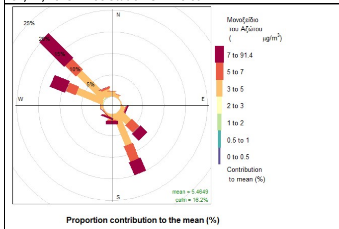
Pollution Rose for NO ( \mu\text{g}/\text{m}^3 ) 01/01/2025 00:00 – 31/12/2025 24:00 Station O.L. Volos
