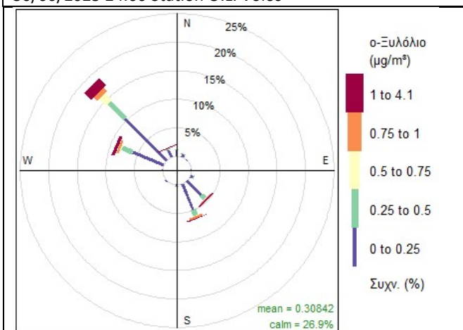
Pollution Rose for o-Xylene ( \mu\text{g}/\text{m}^3 ) 01/01/2025 00:00 – 30/06/2025 24:00 Station O.L. Volos
