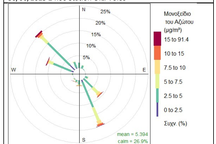
Pollution Rose for NO ( \mu\text{g}/\text{m}^3 ) 01/01/2025 00:00 – 30/06/2025 24:00 Station O.L. Volos
