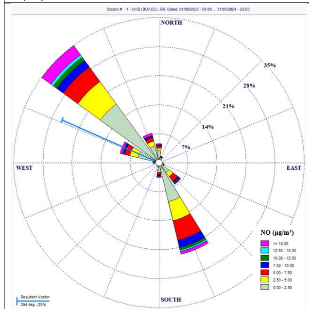
Pollution Rose for NO ( \mu\text{g}/\text{m}^3 ) 01/06/2023 00:00 – 31/05/2024 24:00 Station O.L. Volos AVG: 60min
