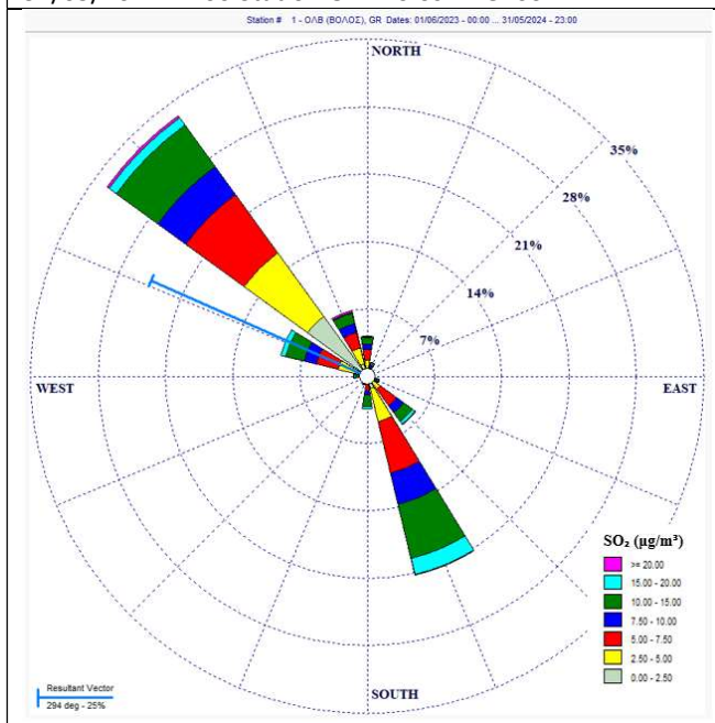
Pollution Rose for SO 2 ( \mu\text{g}/\text{m}^3 ) 01/06/2023 00:00 – 31/05/2024 24:00 Station O.L. Volos AVG: 60min
