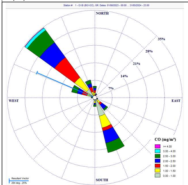
Pollution Rose for CO ( \text{mg}/\text{m}^3 ) 01/06/2023 00:00 – 31/05/2024 24:00 Station O.L. Volos AVG: 60min
