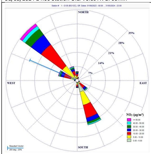
Pollution Rose for NO 2 ( \mu\text{g}/\text{m}^3 ) 01/06/2023 00:00 – 31/05/2024 24:00 Station O.L. Volos AVG: 60min
