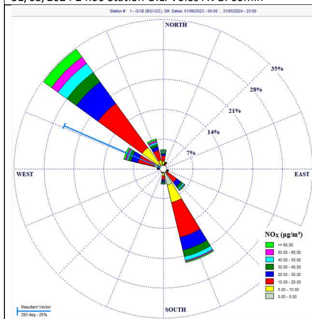
Pollution Rose for NO x ( \mu\text{g}/\text{m}^3 ) 01/06/2023 00:00 – 31/05/2024 24:00 Station O.L. Volos AVG: 60min
