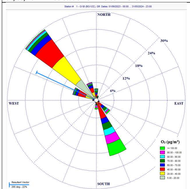
Pollution Rose for Ozone ( \mu\text{g}/\text{m}^3 ) 01/06/2023 00:00 – 31/05/2024 24:00 Station O.L. Volos AVG: 60min
