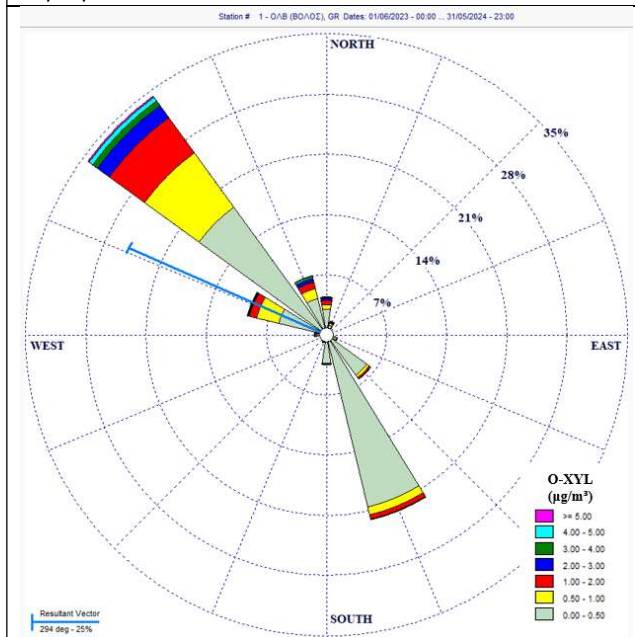
Pollution Rose for o-Xylene ( \mu\text{g}/\text{m}^3 ) 01/06/2023 00:00 – 31/05/2024 24:00 Station O.L. Volos AVG: 60min
