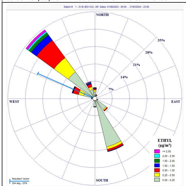
Pollution Rose for EthylBenzene ( \mu\text{g}/\text{m}^3 ) 01/06/2023 00:00 – 31/05/2024 24:00 Station O.L. Volos AVG: 60min
